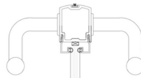
Back to Back (horizontal section) Back to back mounting for aluminum or wood doors
