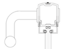
Single Side (horizontal section) End cap mounting for aluminum or wood doors
