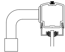
Single Side (horizontal section)
