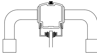
Back to Back (horizontal section)
