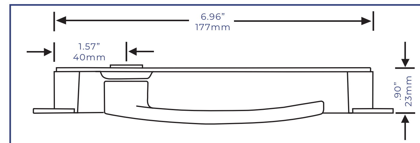
RECESSED HANDLE
